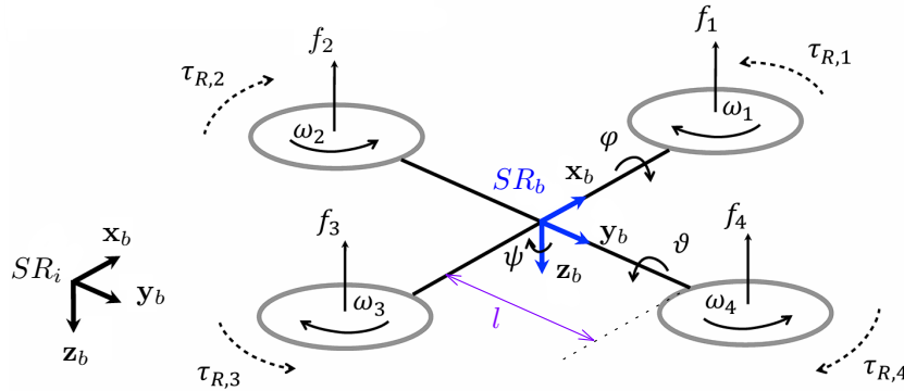
Figure 1.5: Configuration of the quadrotor.
