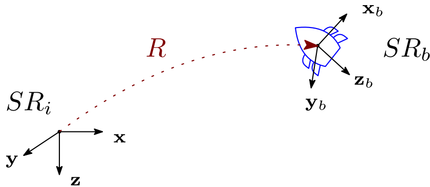
Figure 1.3: SR_b is the reference frame attached to the center of mass of the vehicle, R is the rotation matrix between the two frames.
